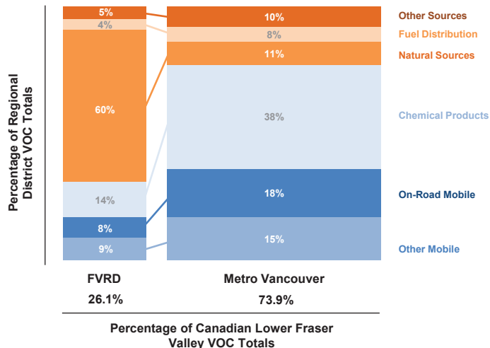
Figure 7: 2010 VOC emissions for the LfV by geographic location and source sector. Note that the width of the bars represents the relative amount of emissions from the two regional districts.
