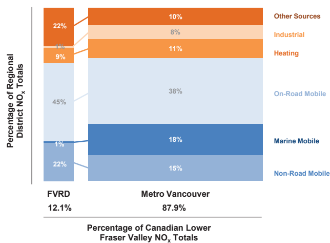
Figure 6: 2010 NO x emissions for the LfV by geographic location and source sector. Note that the width of the bars represents the relative amount of emissions from the two regional districts.
