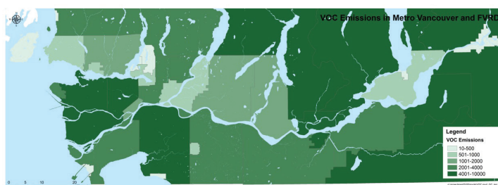
Figure 11: Total VOC emissions in 2010 by municipality
