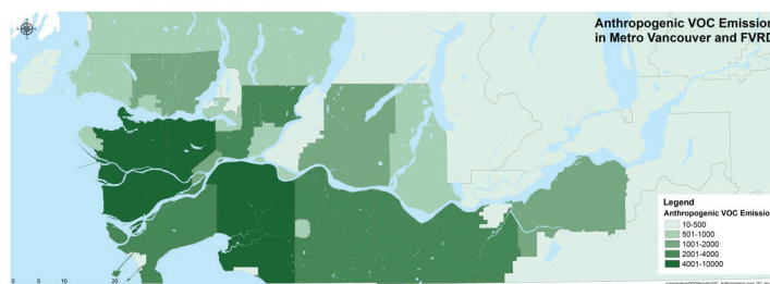
Figure 12: Human-induced VOC emissions in 2010 by municipality
