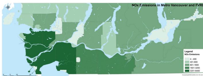
Figure 10: Total NO x emissions in 2010 by municipality
