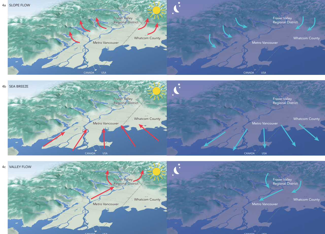
Figure 4 a-c: Summertime peak ozone season day and nighttime airflow patterns in the Canadian Lower Fraser Valley, showing slope flow, sea breeze and valley flow.
